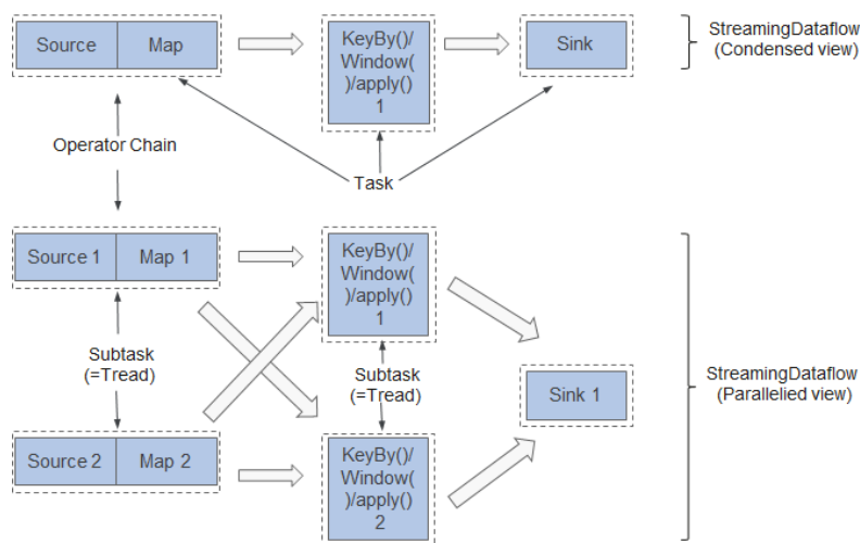
图 1-15 Operator chain
