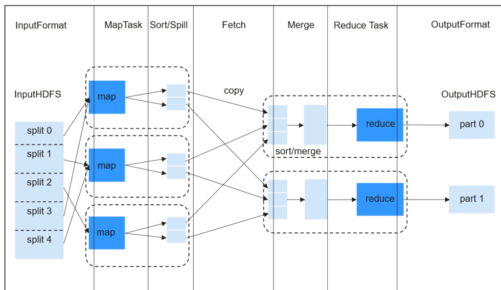
图 1-79 MapReduce job
